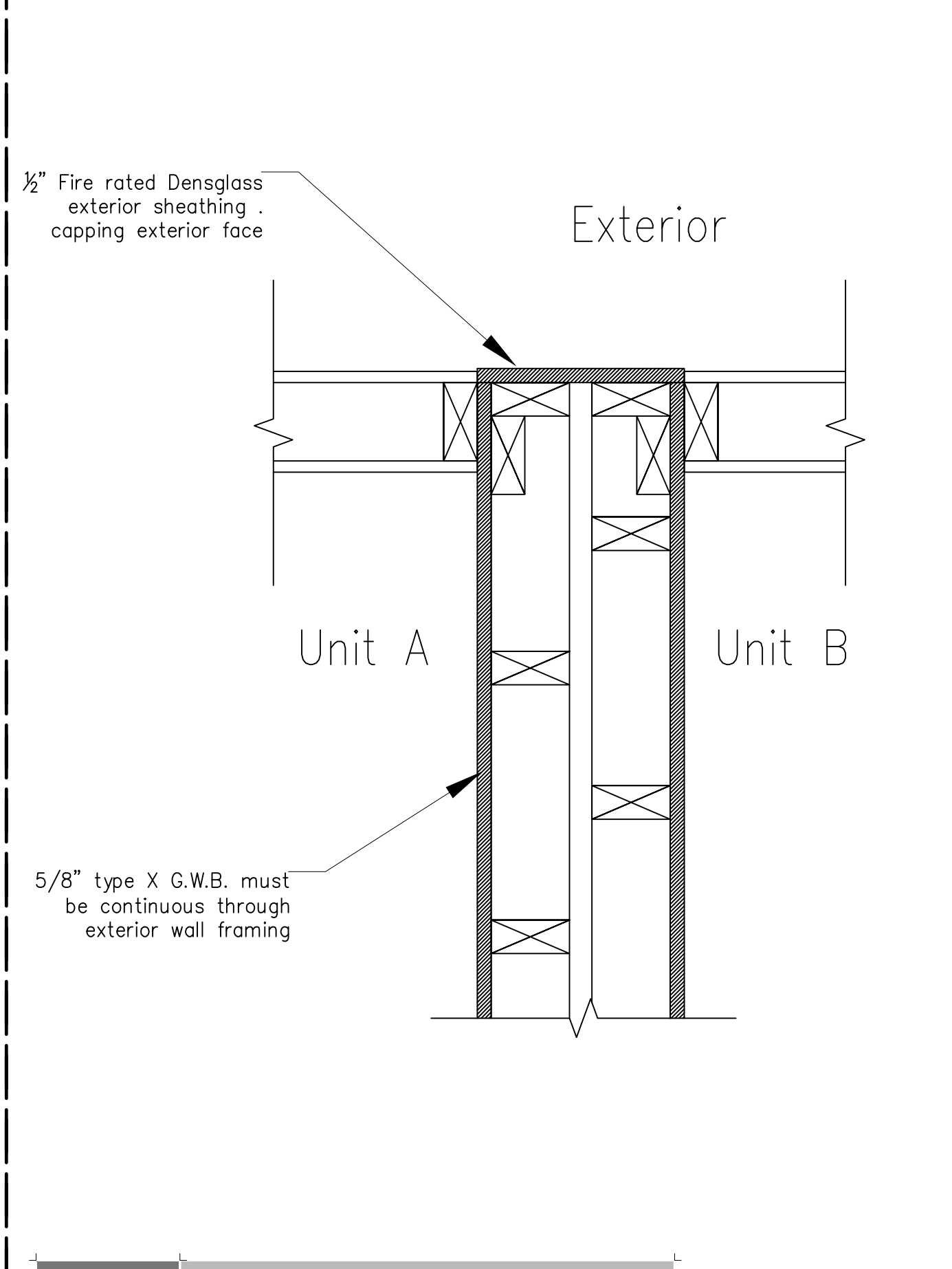
D05 Party Wall Detail - Plan SCALE 1/2" = 1'-0"
