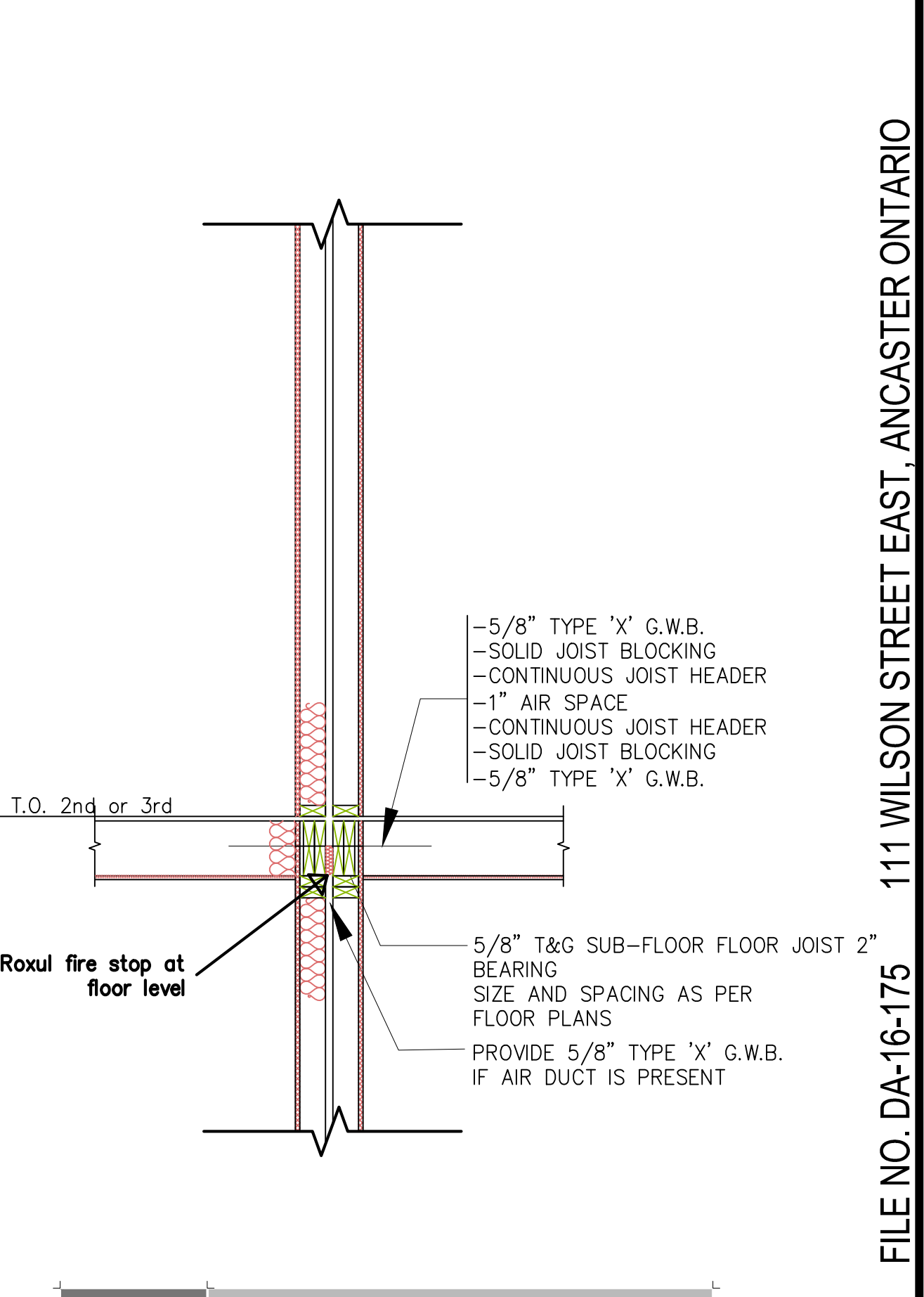
D05 Party Wall Detail SCALE 1/2" = 1'-0"
