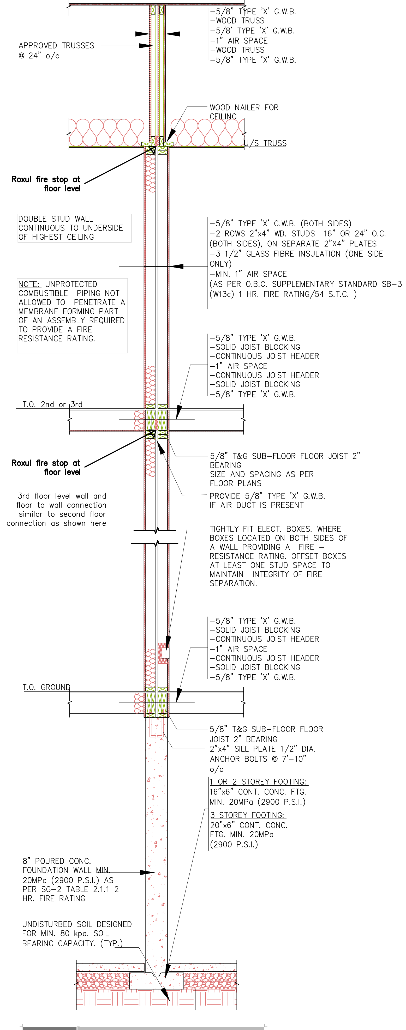
D05 Party Wall Detail SCALE 1/2" = 1'-0"
