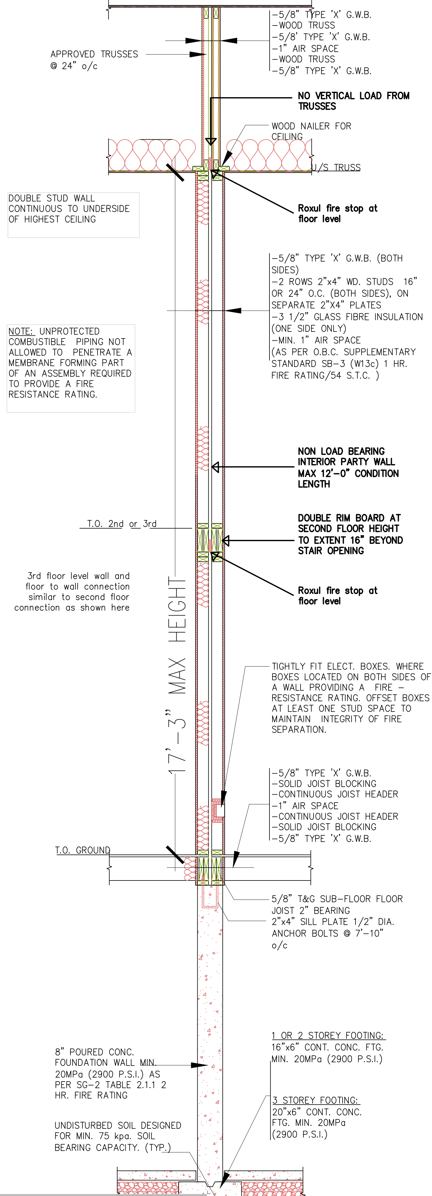
D05a Party Wall Detail SCALE 1/2" = 1'-0"
